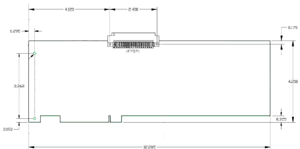
Figure 2 - StreamStor FPDP Connector location
